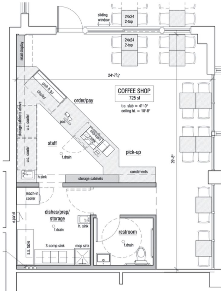
Conceptual Floor Plan - Option 3 - Cafe/Coffee
